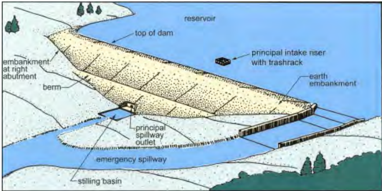
Earthfill Dam
