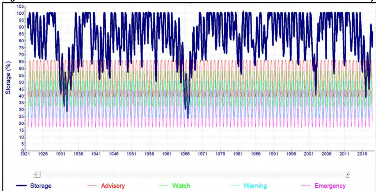
Figure 6 – Reservoir Drawdown with new Streamflow Regulation Releases and w/o Lake Whitney
